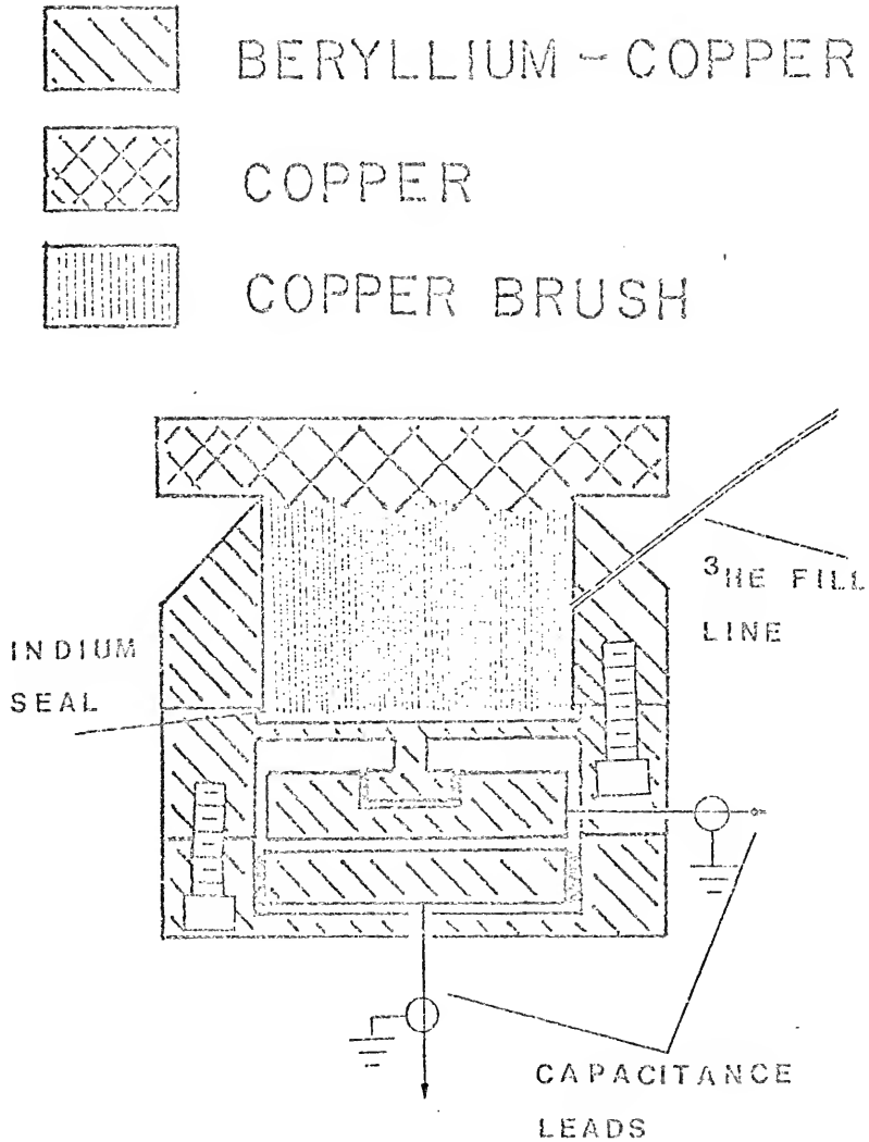
Fig. 5 High Field Pressure Cell.
